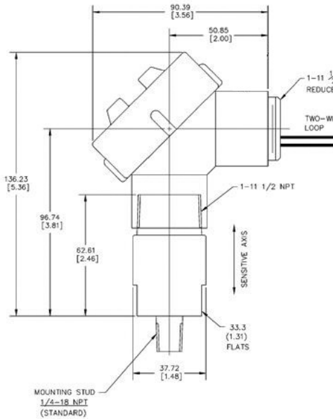
Figure 1: Outline dimensions of the ST5484E (all versions except MIL-Style Connector). Dimensions in mm [inches]. Optional* 8200-001 conduit elbow shown installed.
