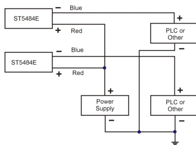
Multiple-transmitter loops
